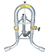
Riser Hydrant
